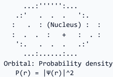
[ QUANTUM MODEL ] (3D Probability Electron Cloud)
